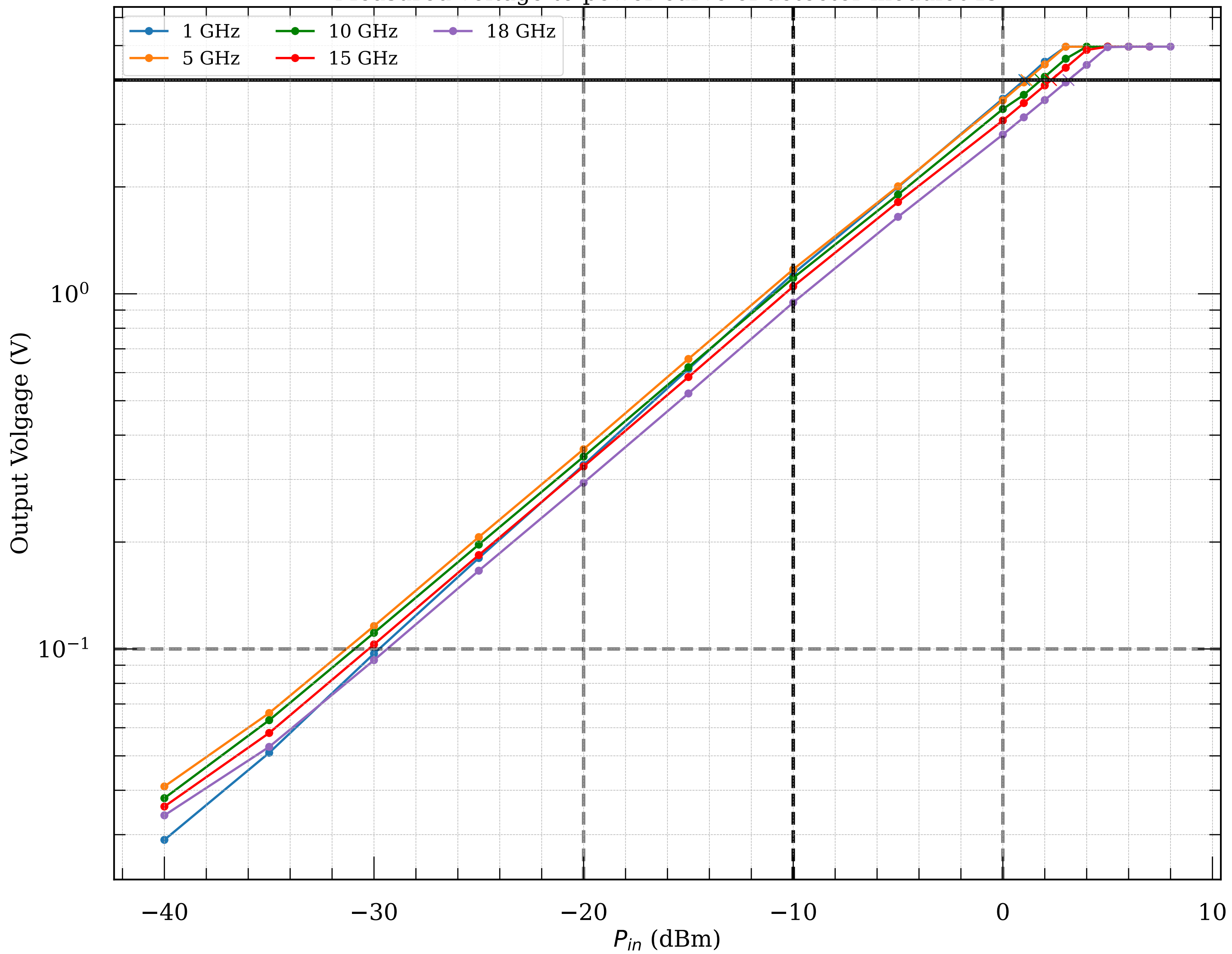
Measured voltage-to-power curve of detector module049
